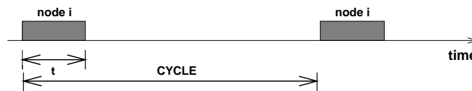
Figure 13: Bandwidth reservation
