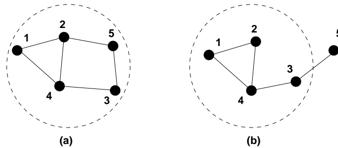
Figure 9: Re-clustering
